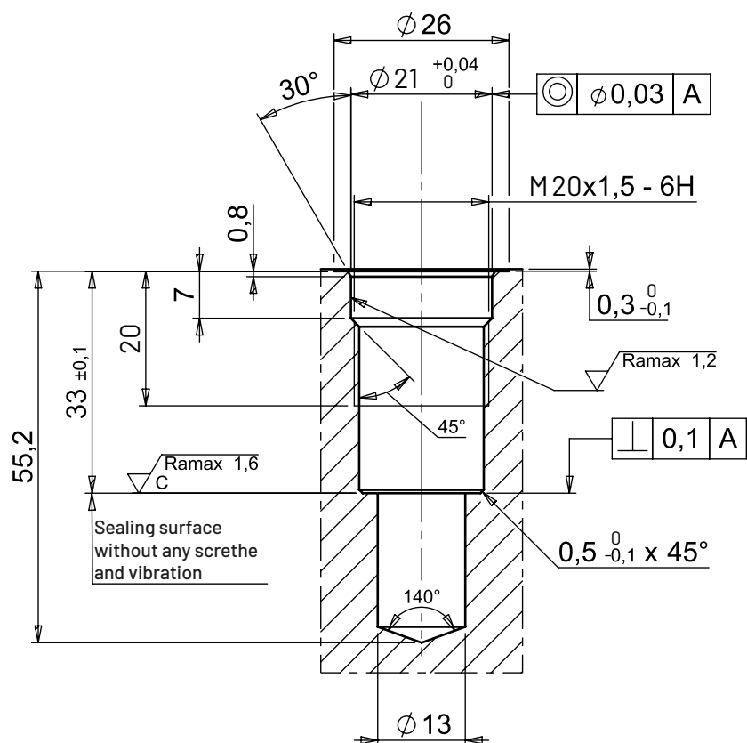
C20 Cavity
