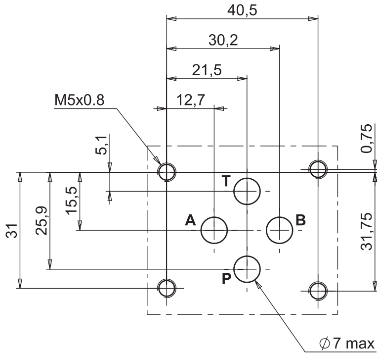
ISO 4401-03 Drilling hole
