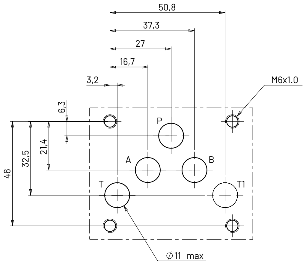
ISO 4401-05 Drilling hole
